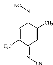
DMe-DCNQI
